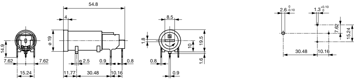
Drilling diagram
