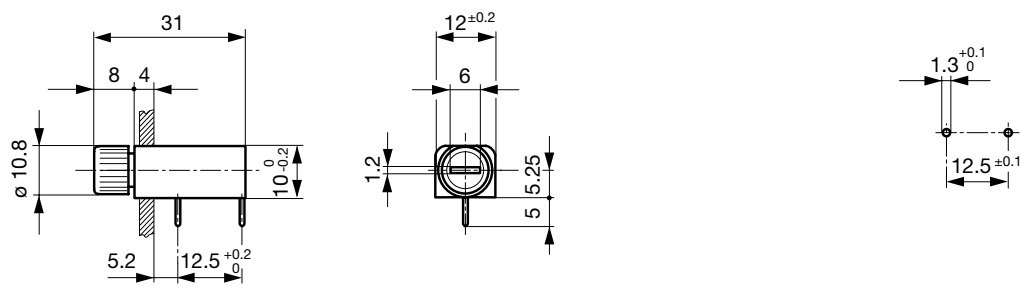
Drilling diagram
