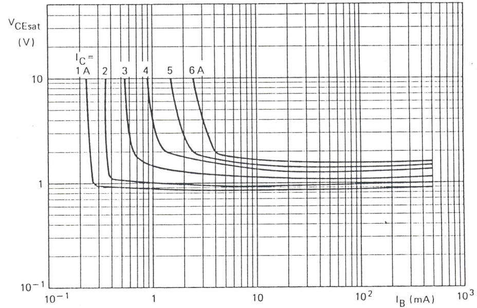
Fig. 17 Typical values collector-emitter saturation voltage. T_j = 25\text{ }^{\circ}\text{C} .
