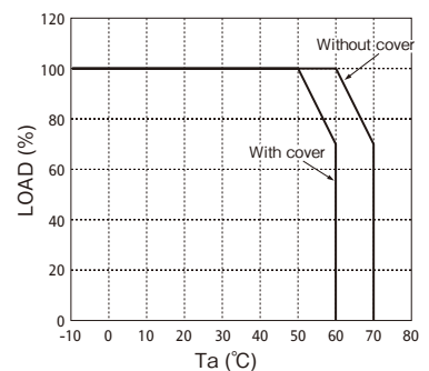
Forced Air Cooling Output Derating Curve
