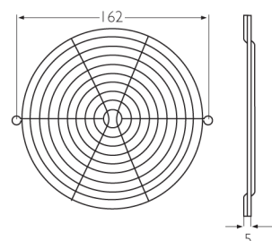
LZ26K Welded steel guard, chromium. 6xxx series fans
