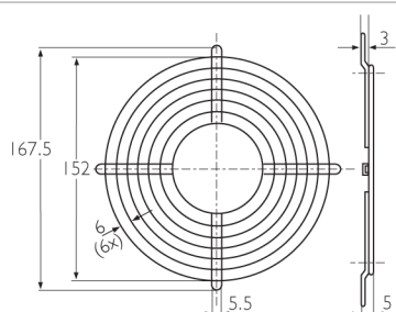
LZ26 Welded steel guard, bright zinc. 6xxx series fans
