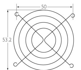
LZ28CP Welded steel guard, chromium. 6xx series fans
