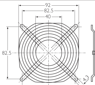
LZ23-I Rust resistant steel wire. 3xxx series fans
