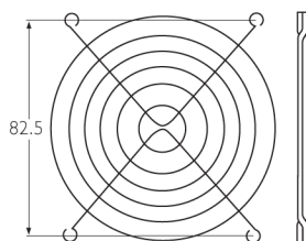
LZ23K Welded steel guard, bright zinc. 3xxx series fans
