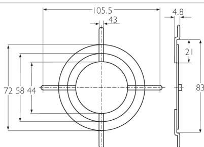
LZ22N Welded steel guard, bright zinc. 8xxx series fans
