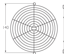
LZ27K Welded steel guard, bright zinc. 7xxx series fans
