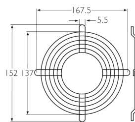
LZ27 Welded steel guard, bright zinc. 7xxx series fans
