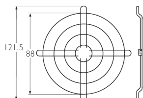
LZ23 Welded steel guard, bright zinc. 3xxx series fans
