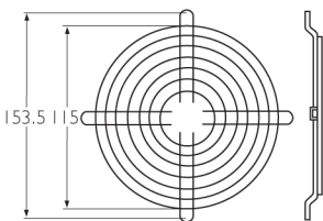
LZ30 Welded steel guard, chromium. 4xxx and 9xxx series fans
