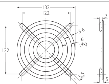
LZ25 Rust resistant steel wire. 5xxx series fans
