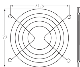
LZ22K Welded steel guard, bright nickel. 8xxx series fans
