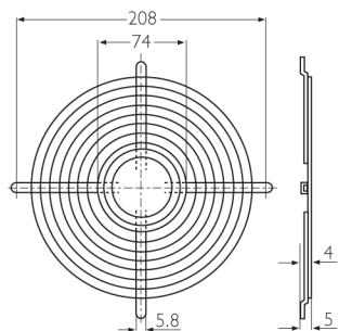
LZ21 Rust resistant steel wire. 2xxx series fans
