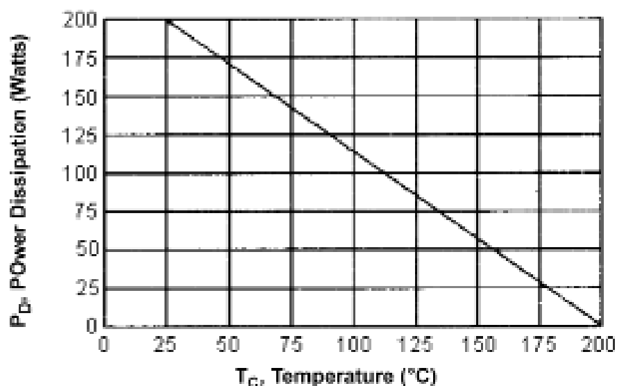
Power Derating
