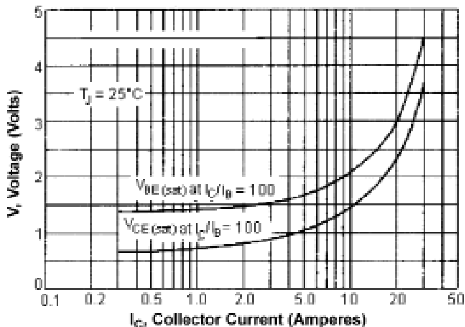
"ON" Voltages
