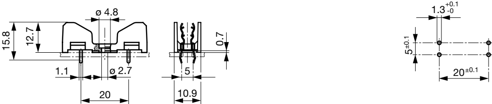
Drilling diagram
