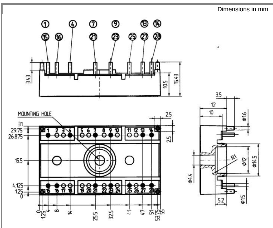
Case T15 (Suggested hole diameter for plastic mounting pins and solder pins in the PCB: 2mm)
