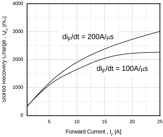
Figure 20. Stored Charge
