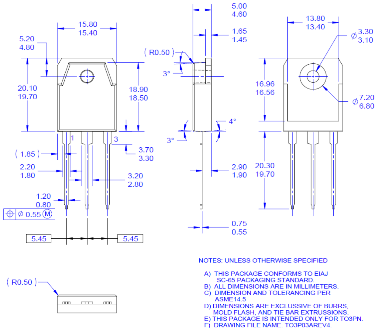
Figure 22. TO-3P 3L - 3LD, T03, PLASTIC, EIAJ SC-65
