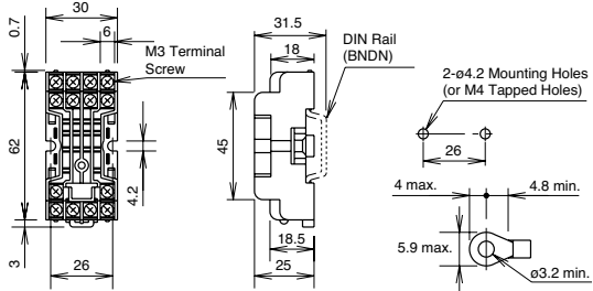
Terminal Arrangement
