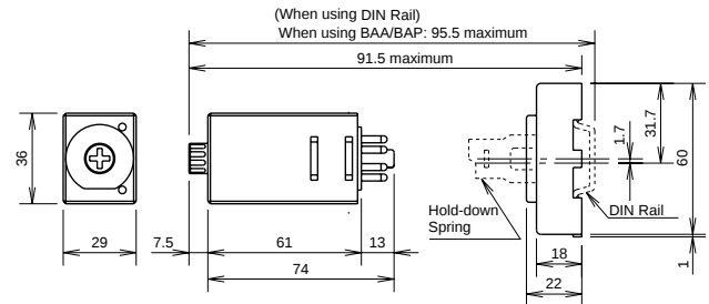
GT5P Timer, 8-Pin with SR2P-06
