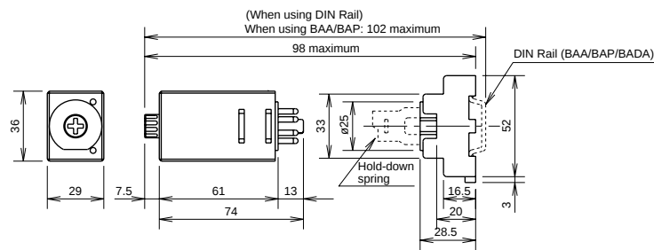
GT5P Timer, 8-Pin with SR2P-05
