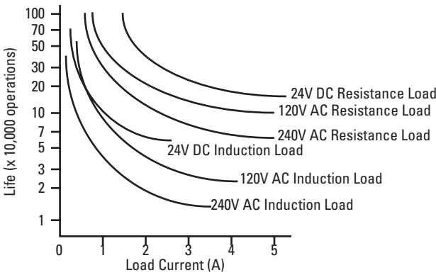
Electrical Life Curves
