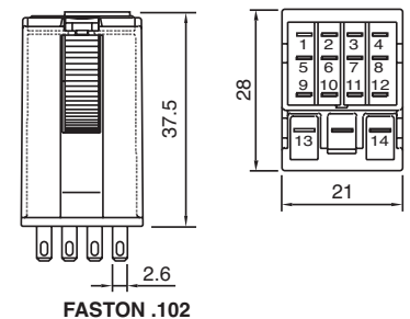
fig. 4. Dimension (mm)
