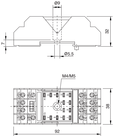
Dimensions (mm)
