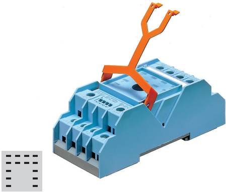
Connection diagram
