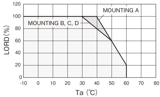
HWS100/A
