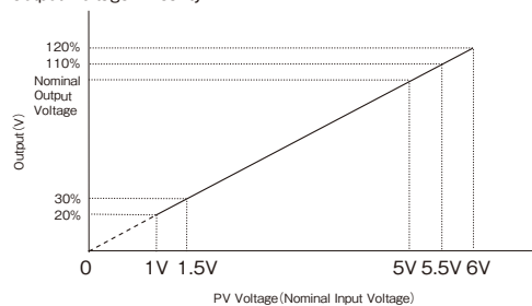
Output Voltage Linearity
