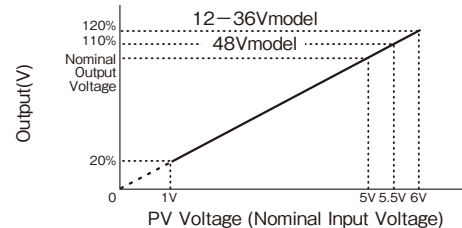
Output Voltage Linearity
