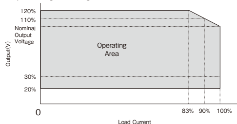
Output Voltage Derating
