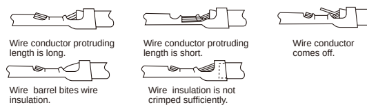
Fig.2: Examples of defective crimping
