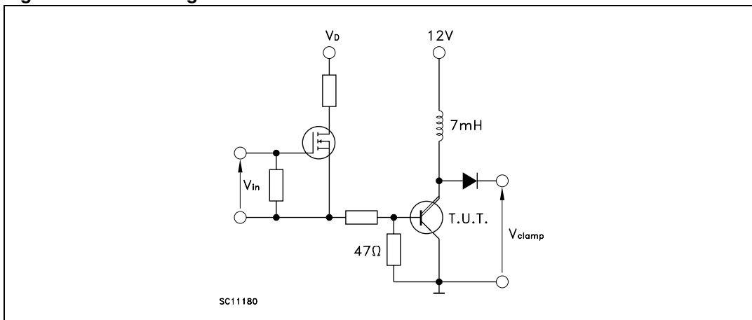
Figure 13. Switching time test circuit
