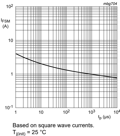
Fig. 2. Non-repetitive peak forward current as a function of pulse duration; typical values
