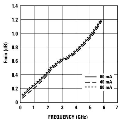
Figure 18. F_{min}^{[1]} vs. Frequency and I_{ds} at 3V.
