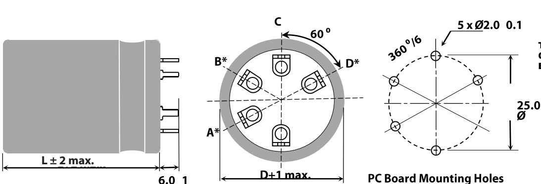
PC Board Mounting Holes
