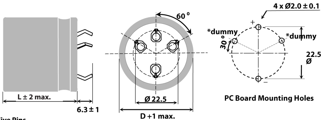
PC Board Mounting Holes
