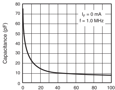
Fig. 8 - Switch Capacitance vs. Applied Voltage
