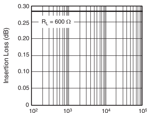
Fig. 9 - Insertion Loss vs. Frequency
