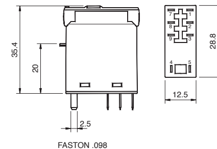
fig. 4. Dimension (mm)
